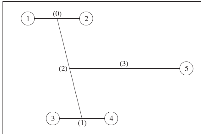
Fig. 1. The hierarchical structure of the stellar system for KOREL.
